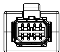
MATING SHAPE : TYPE I 2201855-1/-2/-3/-6 SCALE 3:1
